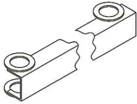
Artikel No. 4040/41 ... 4080/81 SIDE BAR galvanised/stainless steel
