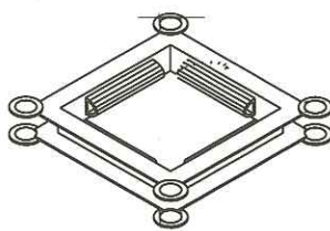
Artikel No. 4518 INNER PILE CAGE 4 plastic fenders including screw joint units, galvanised
