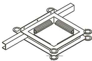
Artikel No. 4512 PILE CAGE 2L 4 plastic fenders including screw joint units, galvanised
